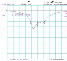
Return Loss : -12.43 dB
