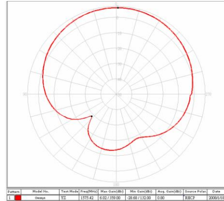
YZ Plane 1575.42 MHz
