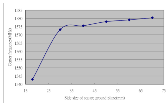
Graph of 18.5mm Patch Centre Frequency shift with Ground-plane size
