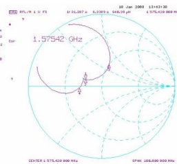
Impedance : 31.28+j6.33 Ohm
